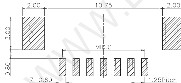
RECOMMENDER P.C.B LAYOUT TOP VIEW (GENERAY TOLERANCE \pm 0.10 )
